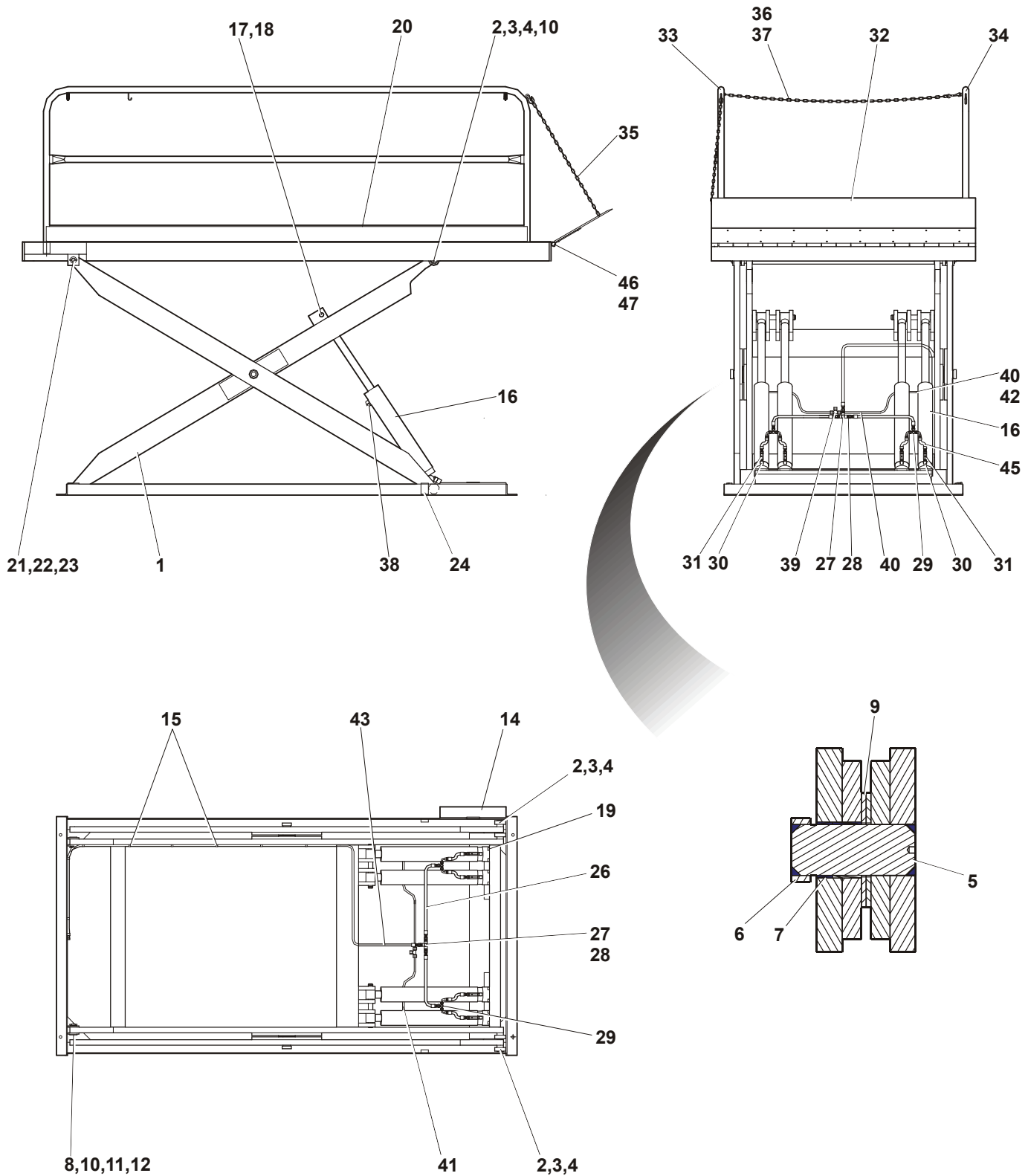
Figure 15 : General Assembly - 5, & 6,000 - 120" Deck Length
