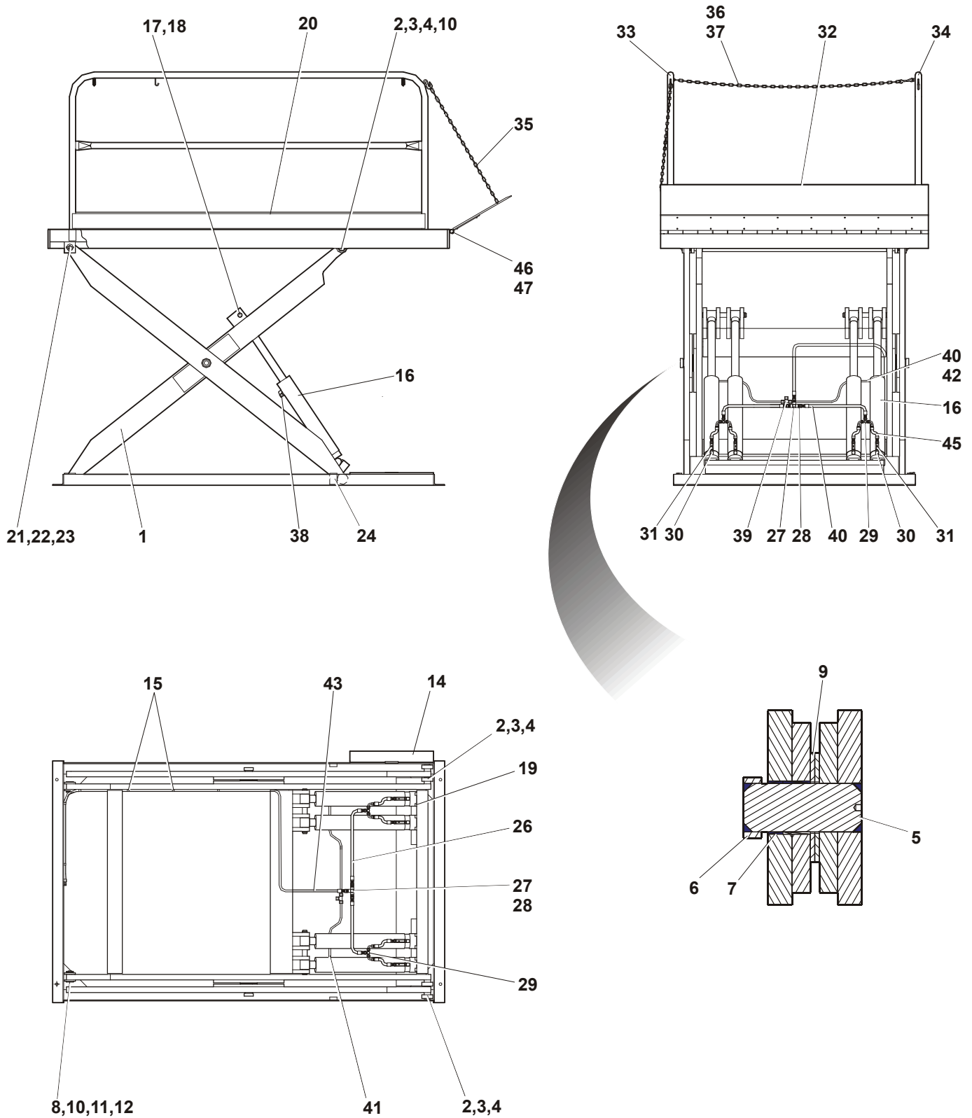
Figure 11 : General Assembly - 6,000 lb. - 108" Deck Length
